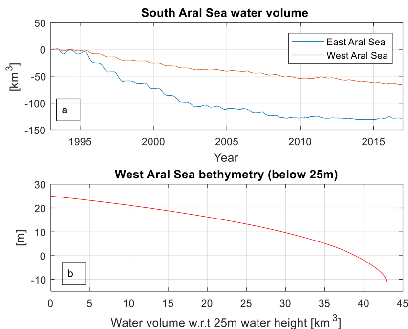
Figure 4. (a) the South Aral Sea volume variations and (b) the West Aral Sea bathymetry below 25 m MSL.
